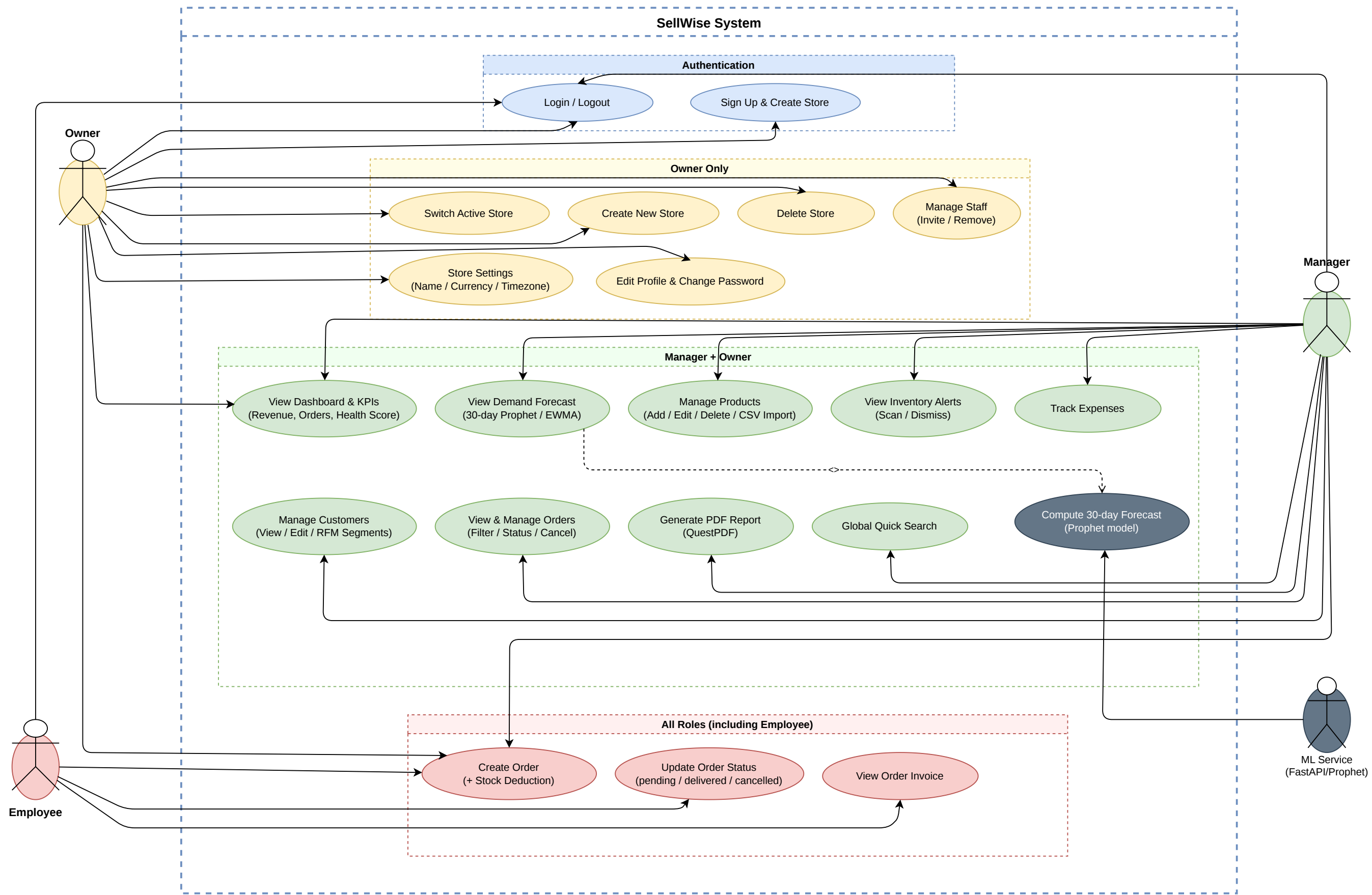
SellWise - Use Case Diagram
